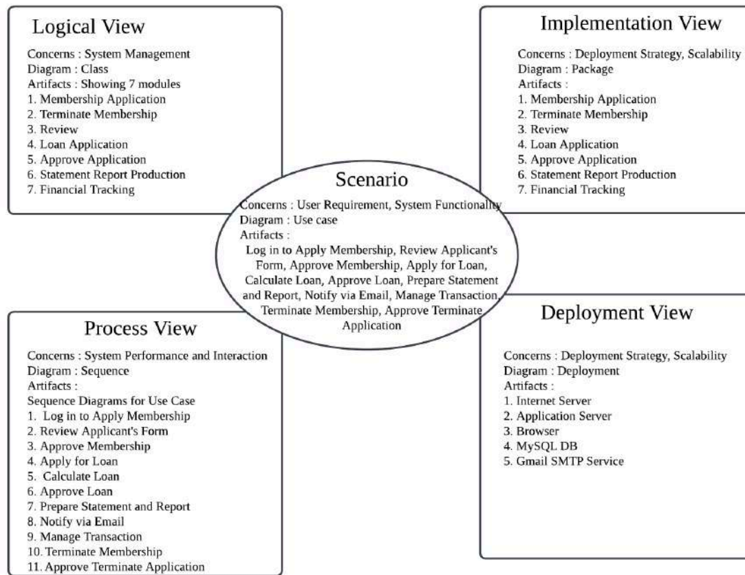
Figure 2.1: 4+1 Architectural View Model
